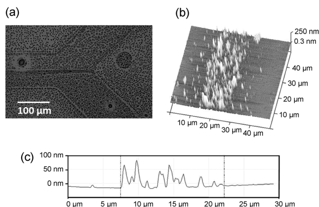
Figure 3. Two-phase laminar flow patterned AMP film prepared with flow rate = 0.2 \text{ mL min}^{-1} and flow time = 60 min. a) Optical micrograph of water condensation figure; b) 3D AFM image; c) single line profile.
